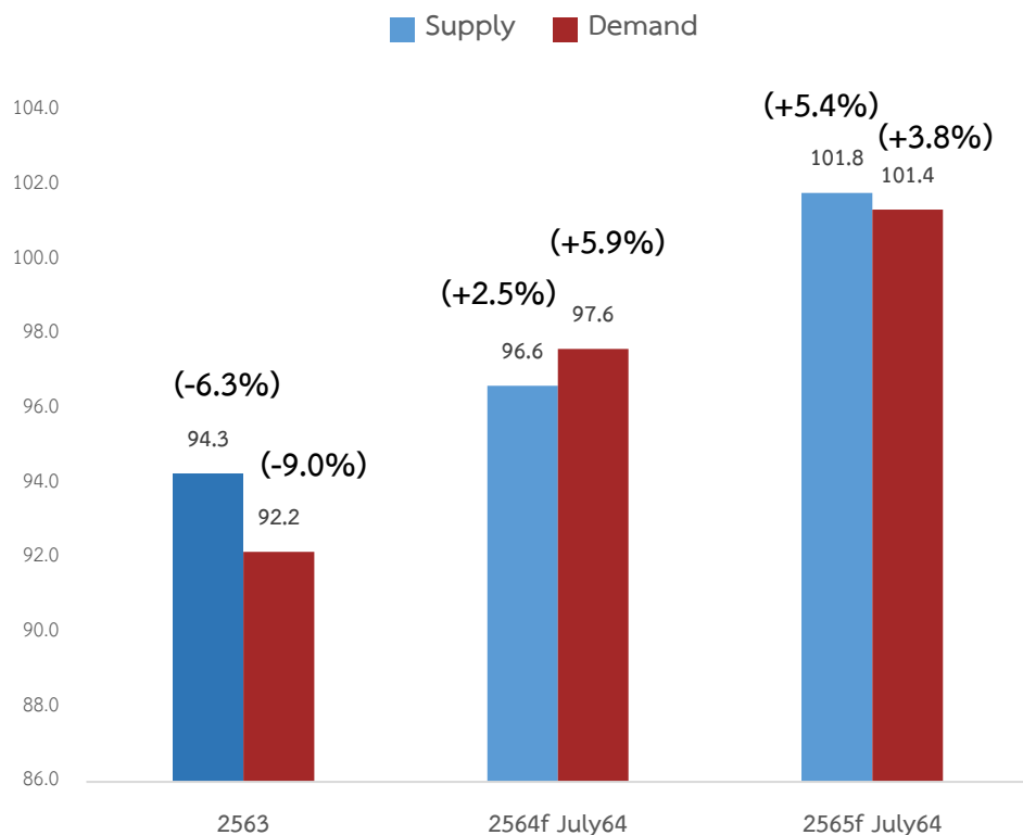
EIA Forecast
